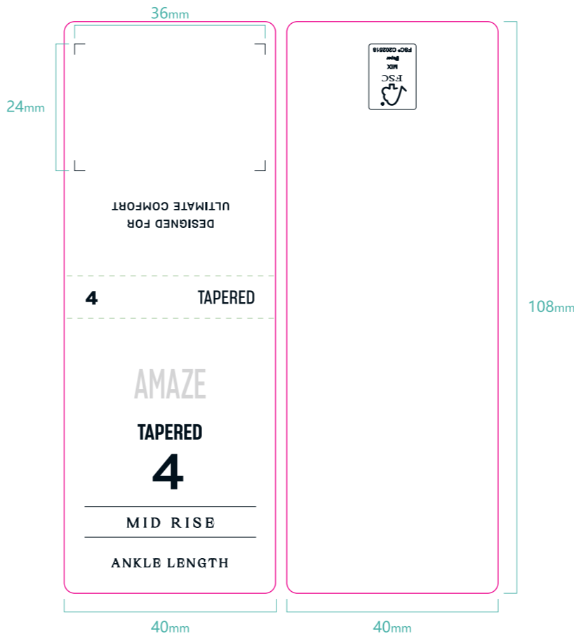
AMAZE WAIST BAND TAG 40mmx108mm JJW-AM-WT
